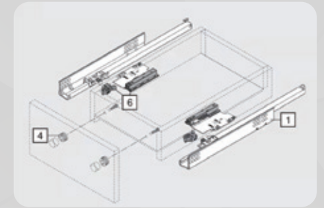
Guiding rail of drawer
